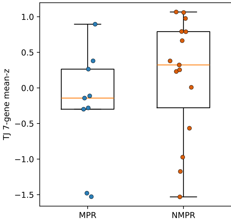
GSE207422 TJ 7-gene vs pathologic MPR vs NMPR
