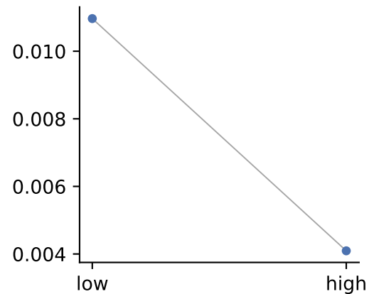
CXCL10_CXCR3 n=1
