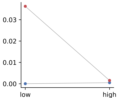
CCL5_CCR5 n=2
