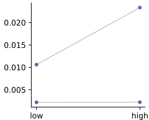
CCL5_CCR5 n=2
