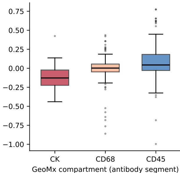
T+B score
