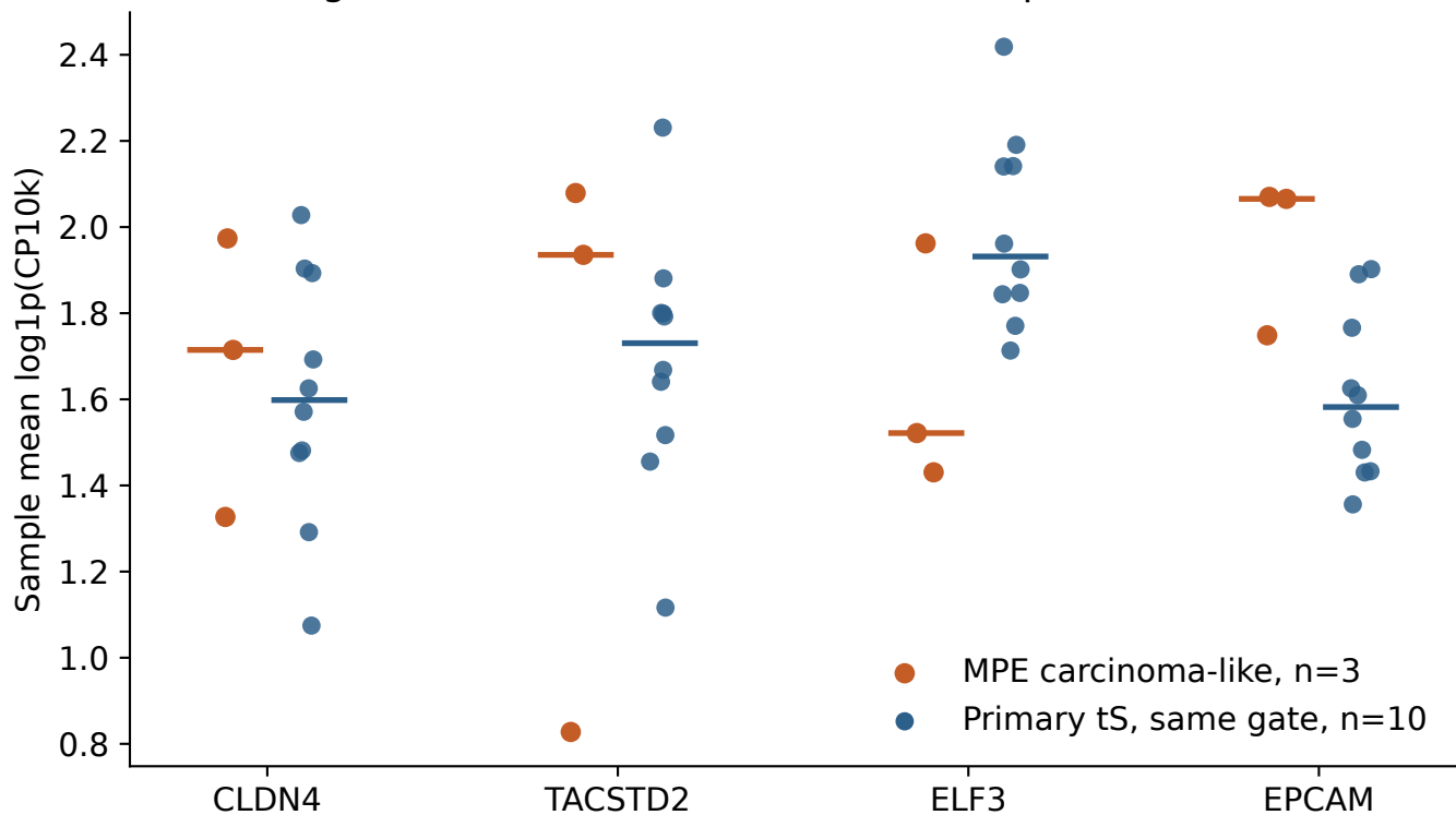
Same gate (EPCAM+ WT1- CALB2-), samples with \geq 20 cells
