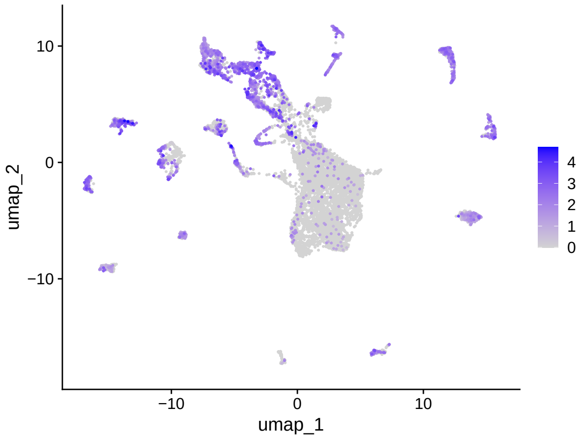
Harmony UMAP – CLDN4 (log-norm)
