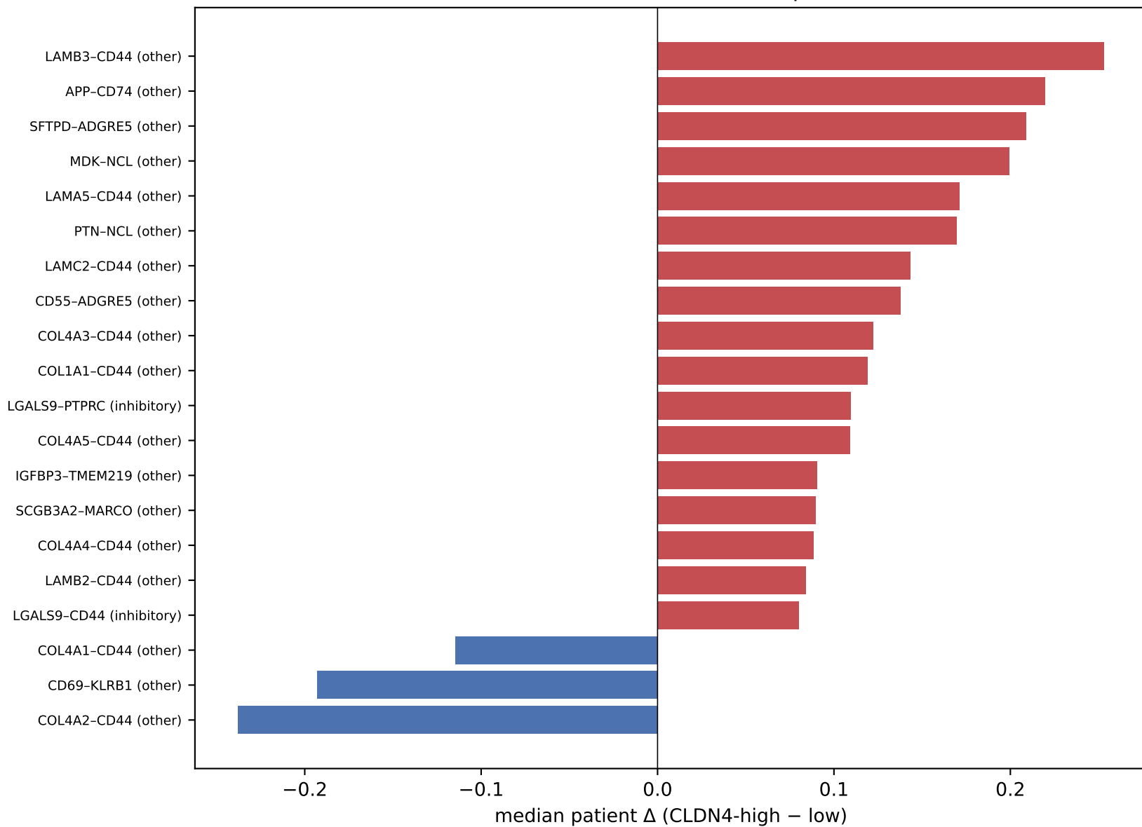
cellchat T/NK median: median patient \Delta
