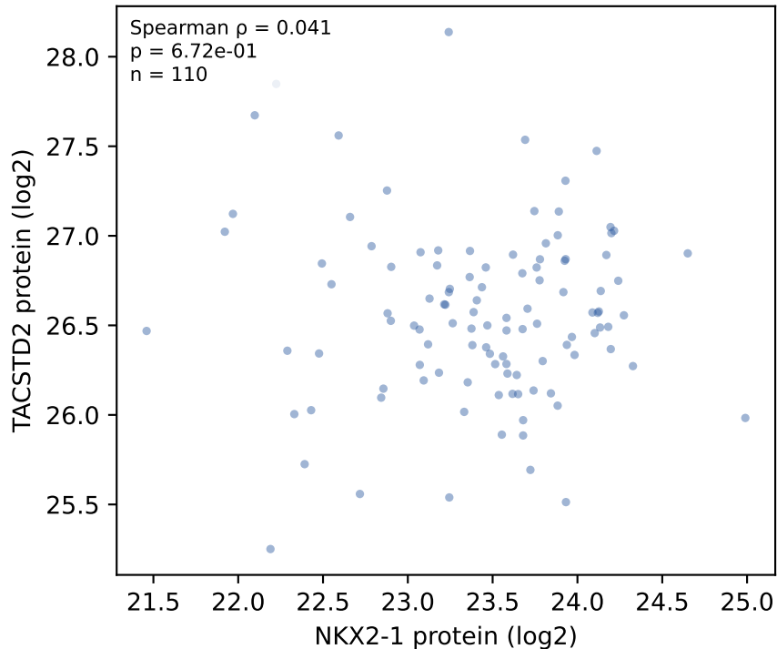
CPTAC-LUAD protein NKX2-1 vs TACSTD2
