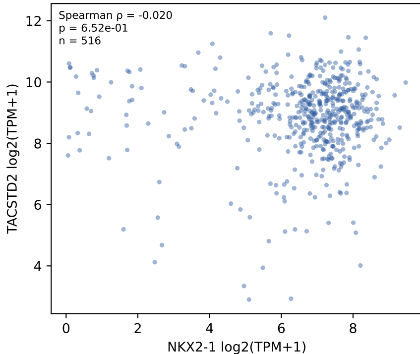
TCGA-LUAD NKX2-1 vs TACSTD2
