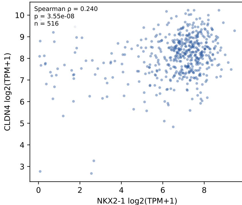
TCGA-LUAD NKX2-1 vs CLDN4
