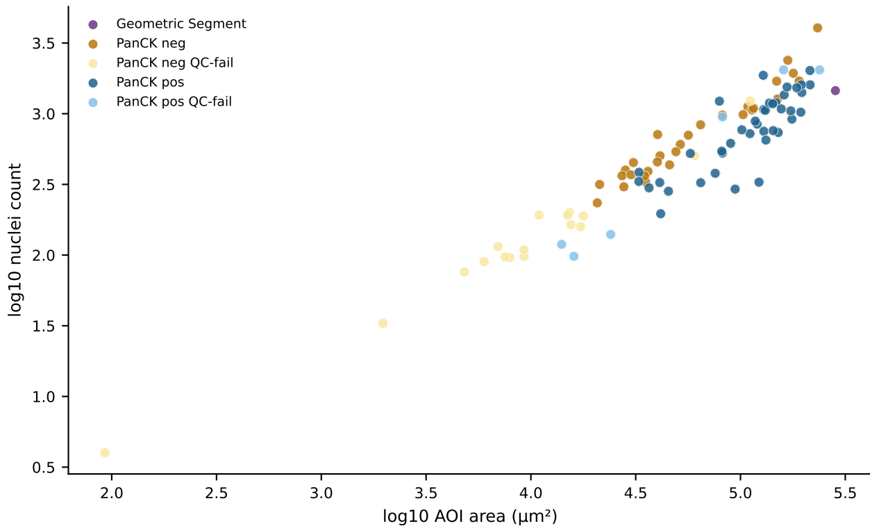
ROI / AOI size and nuclei (GEO metadata)
