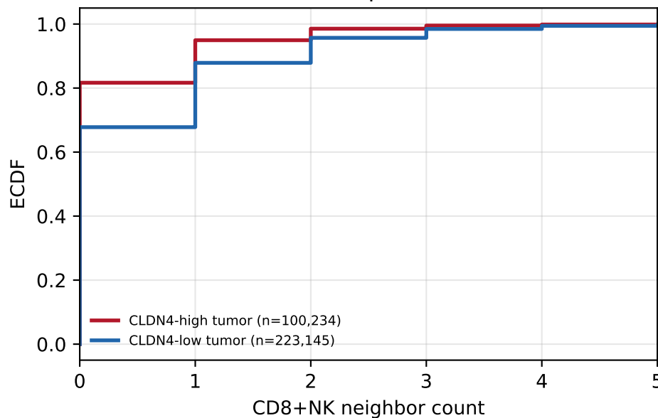
CD8+NK neighbor counts around CLDN4-high vs low tumor (8 sections)
