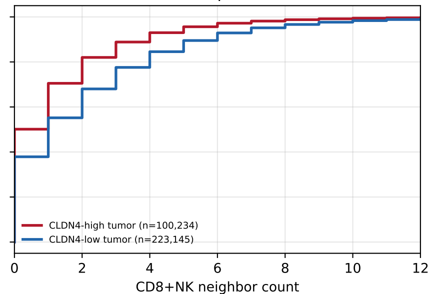
CD8+NK neighbor counts around CLDN4-high vs low tumor (8 sections)
