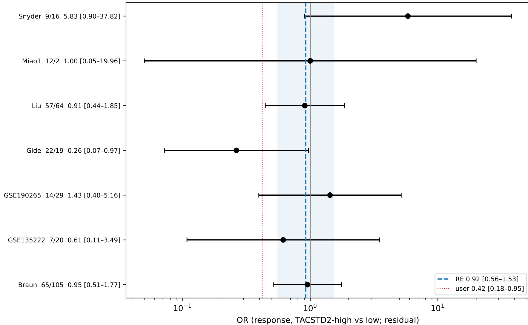
all_open_DCB | TACSTD2 residual median | DCB | k=7
