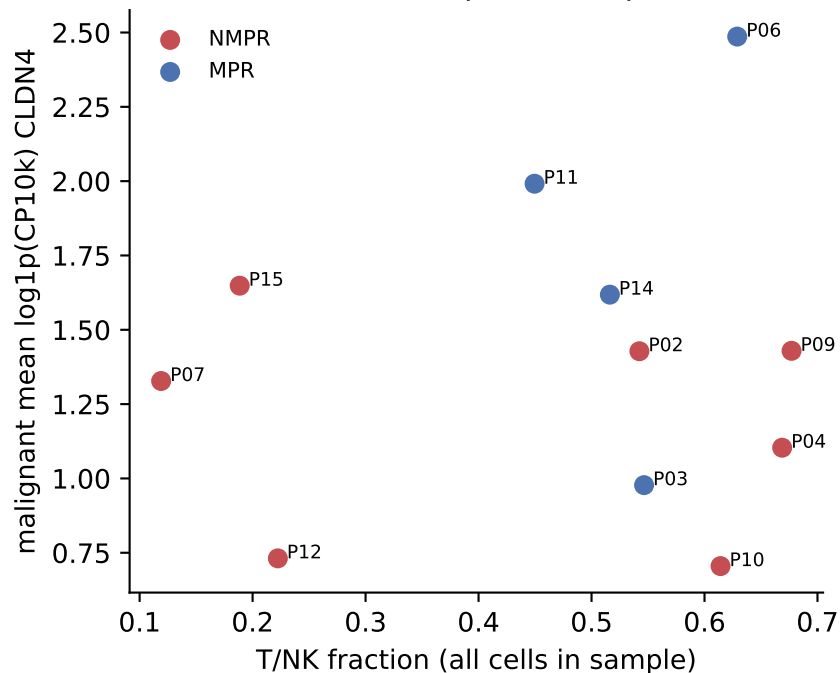
vs T/NK fraction \rho = -0.055 p = 0.873
