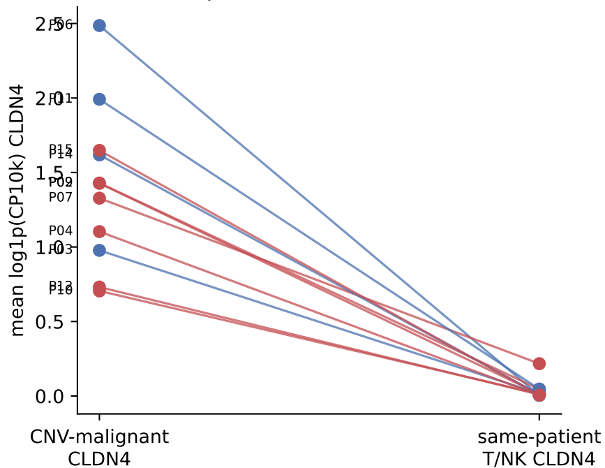
GSE207422 post, inferCNV-like p95 n=11 patients with \geq 5 cells/arm
