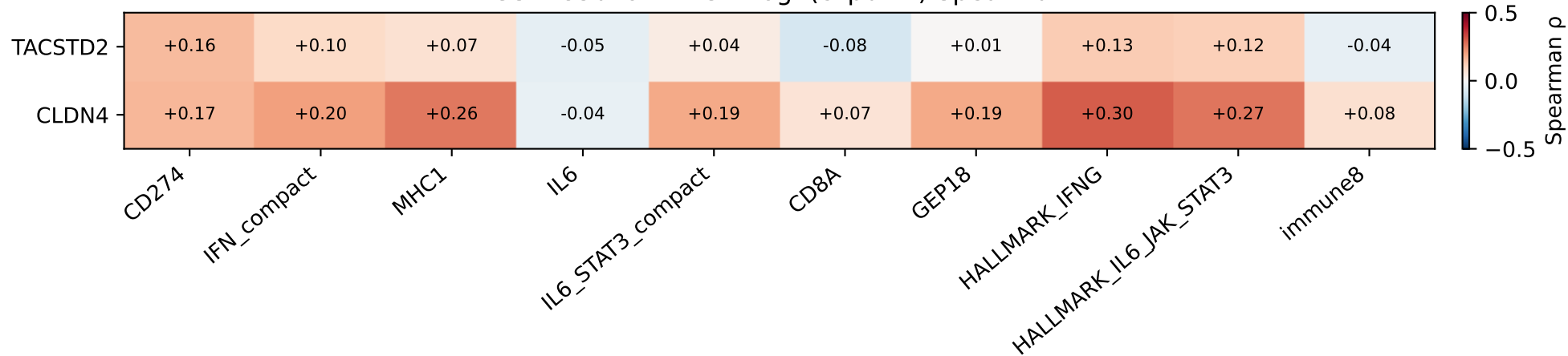
GSE285029 n=234 log2(clip0+1) Spearman
