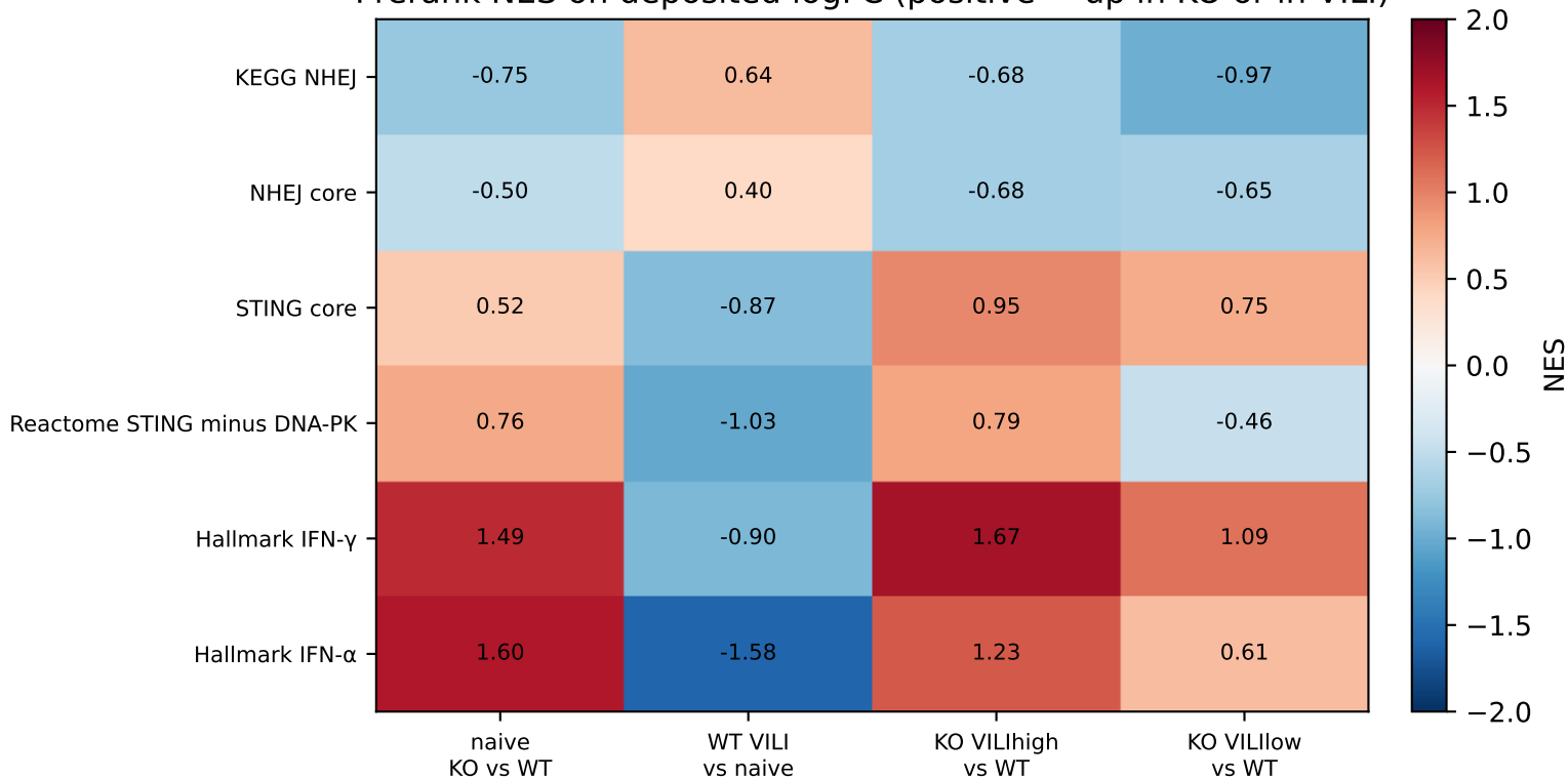
Prerank NES on deposited logFC (positive = up in KO or in VILI)
