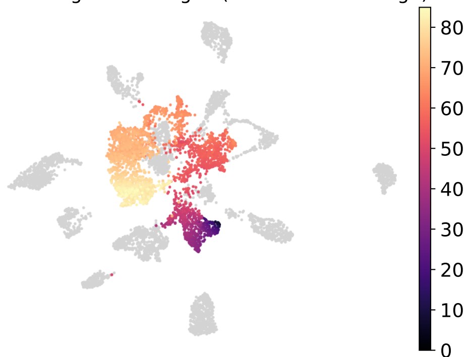
UMAP Slingshot Lineage1 (root not CLDN4-high)
