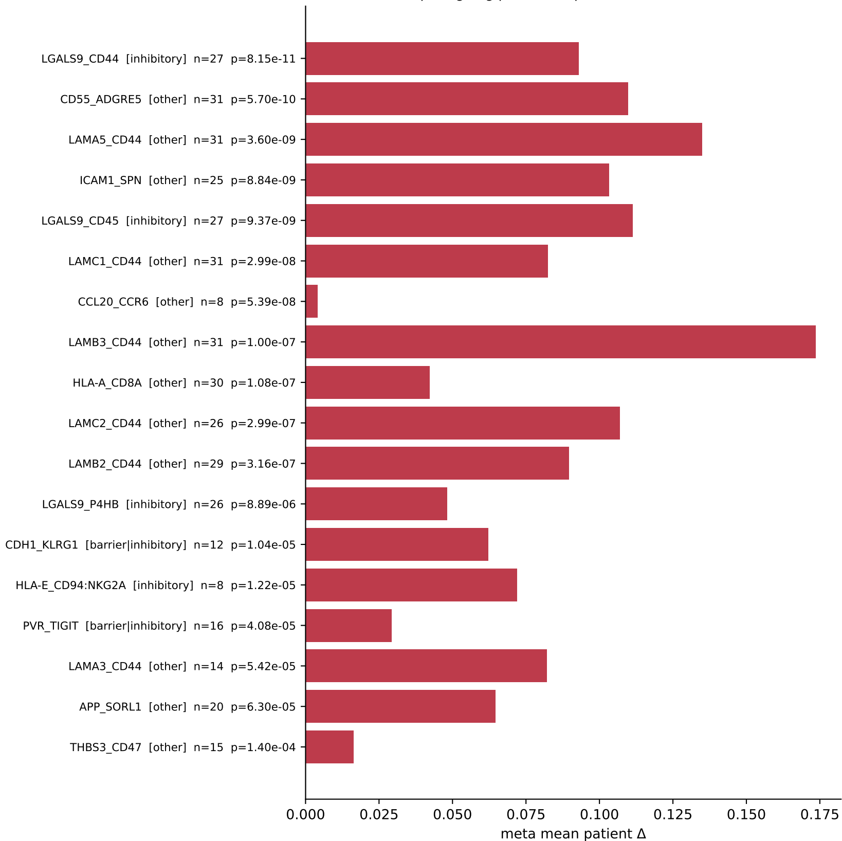
Extra: top outgoing patient- \Delta P pairs (CellChat Q4 vs Q1, n \geq 8 )
