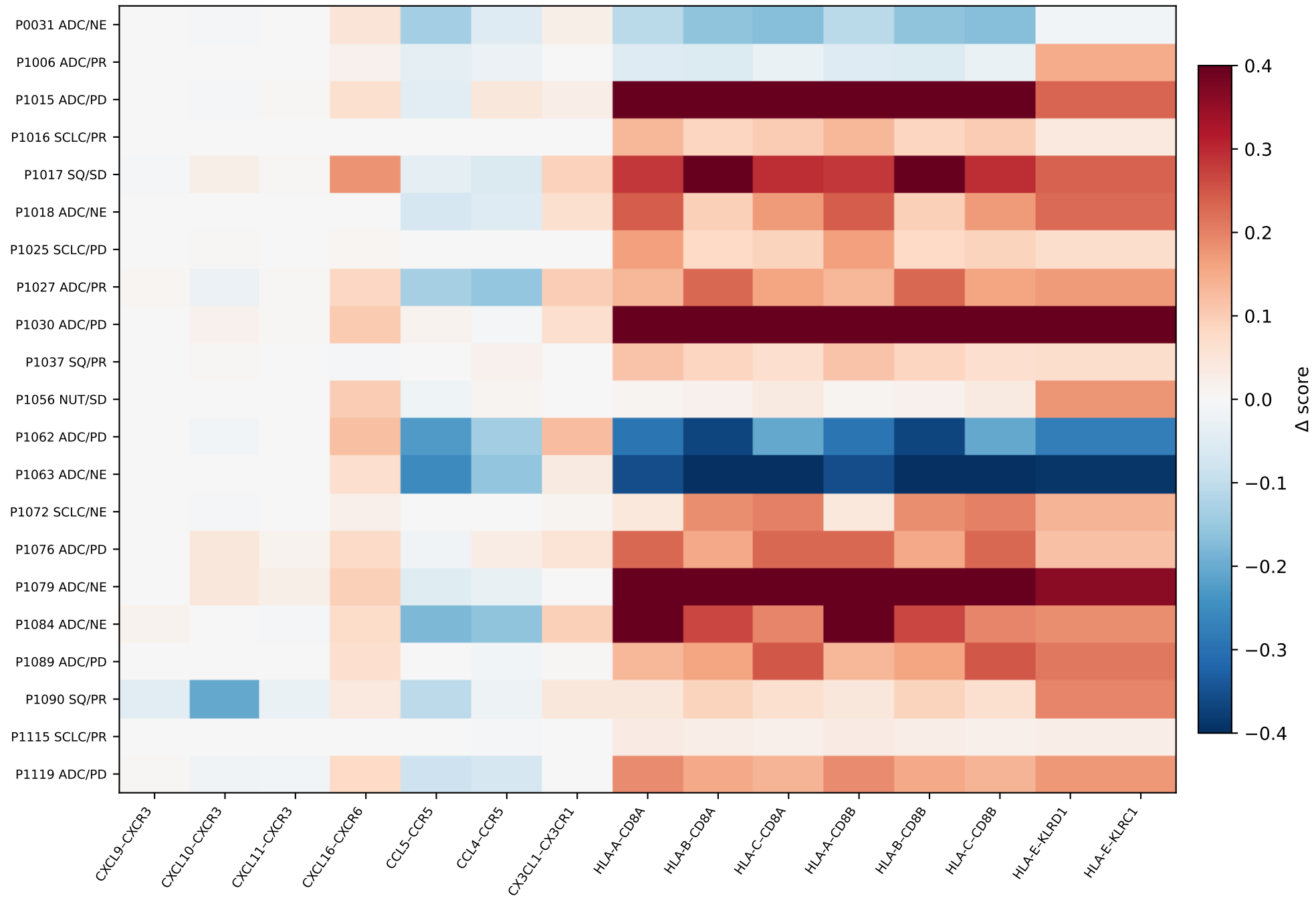
Extra: per-patient outgoing \Delta (CLDN4-high – low)
