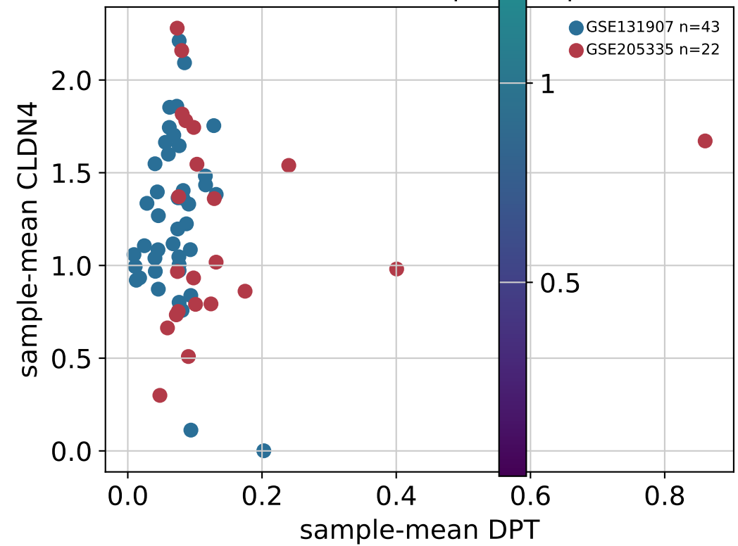
CLDN4 vs DPT n=65 \rho=0.08 p=0.538
