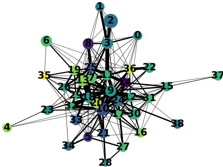
PAGA (Leiden) colored by mean CLDN4
