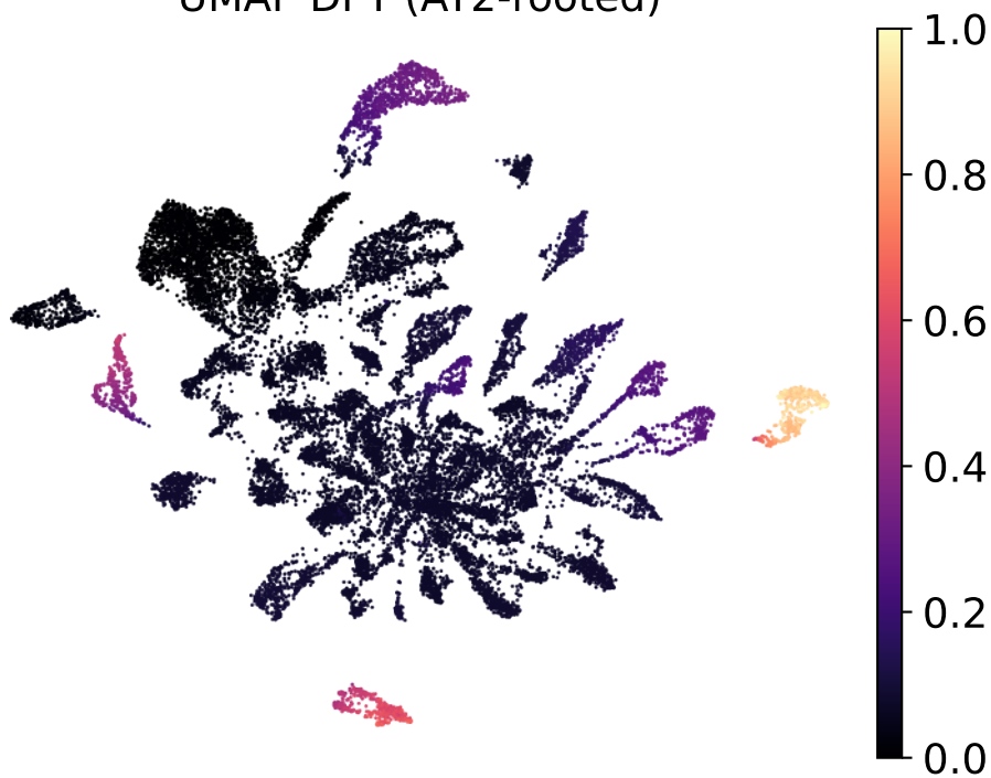
UMAP DPT (AT2-rooted)
