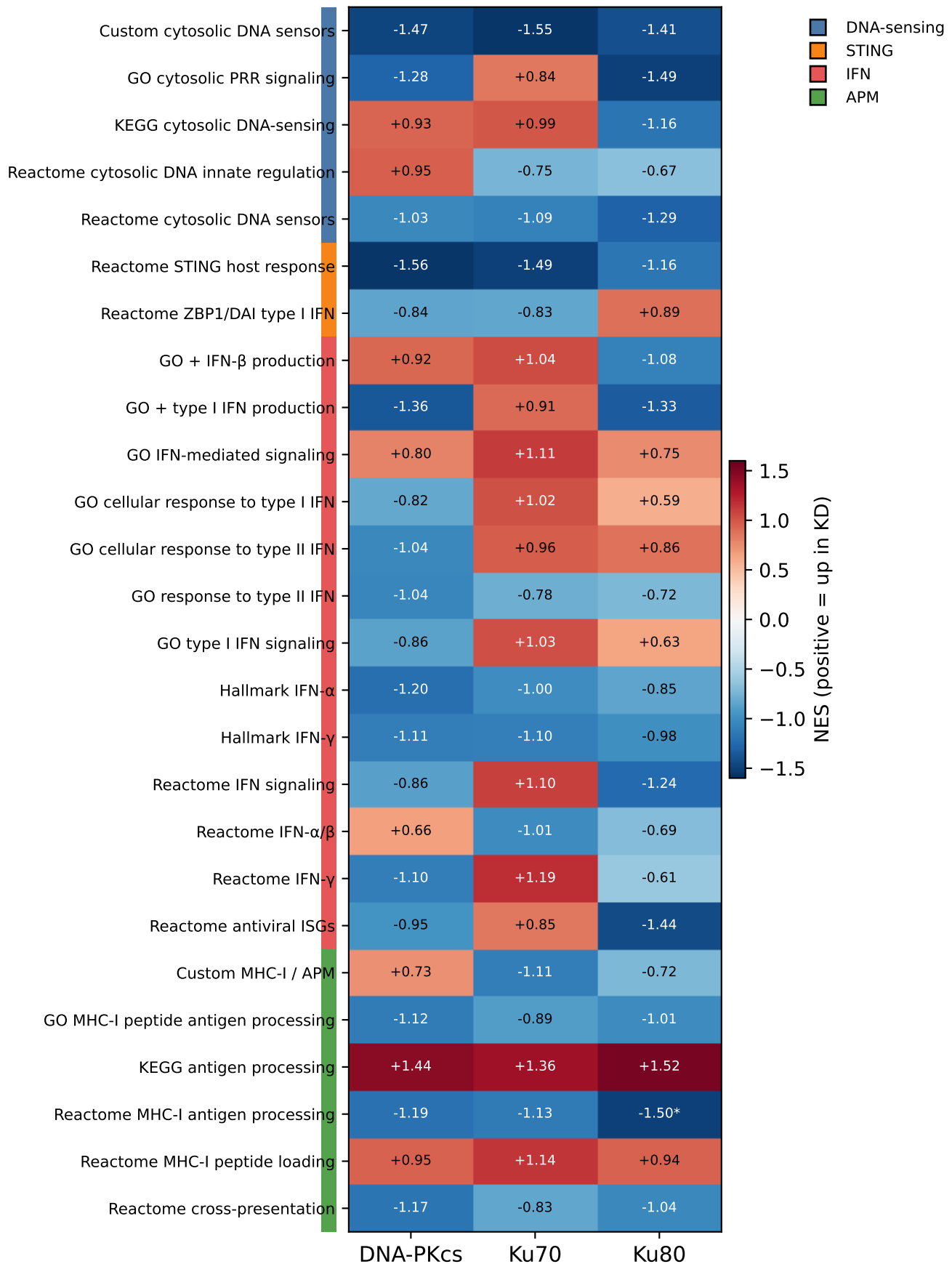
GSE180581 prerank NES KD minus matched siControl (* BH-FDR < 0.05 within panel)
