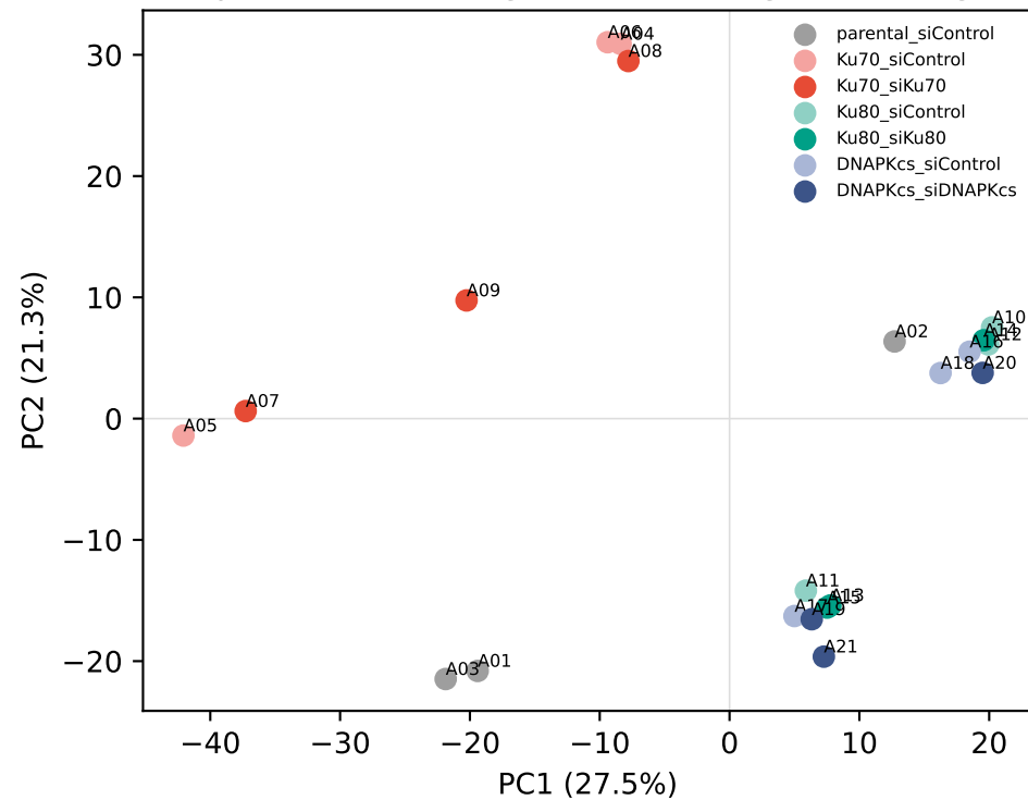
Top 2000 variable genes with range \geq 0.5 \log_2
