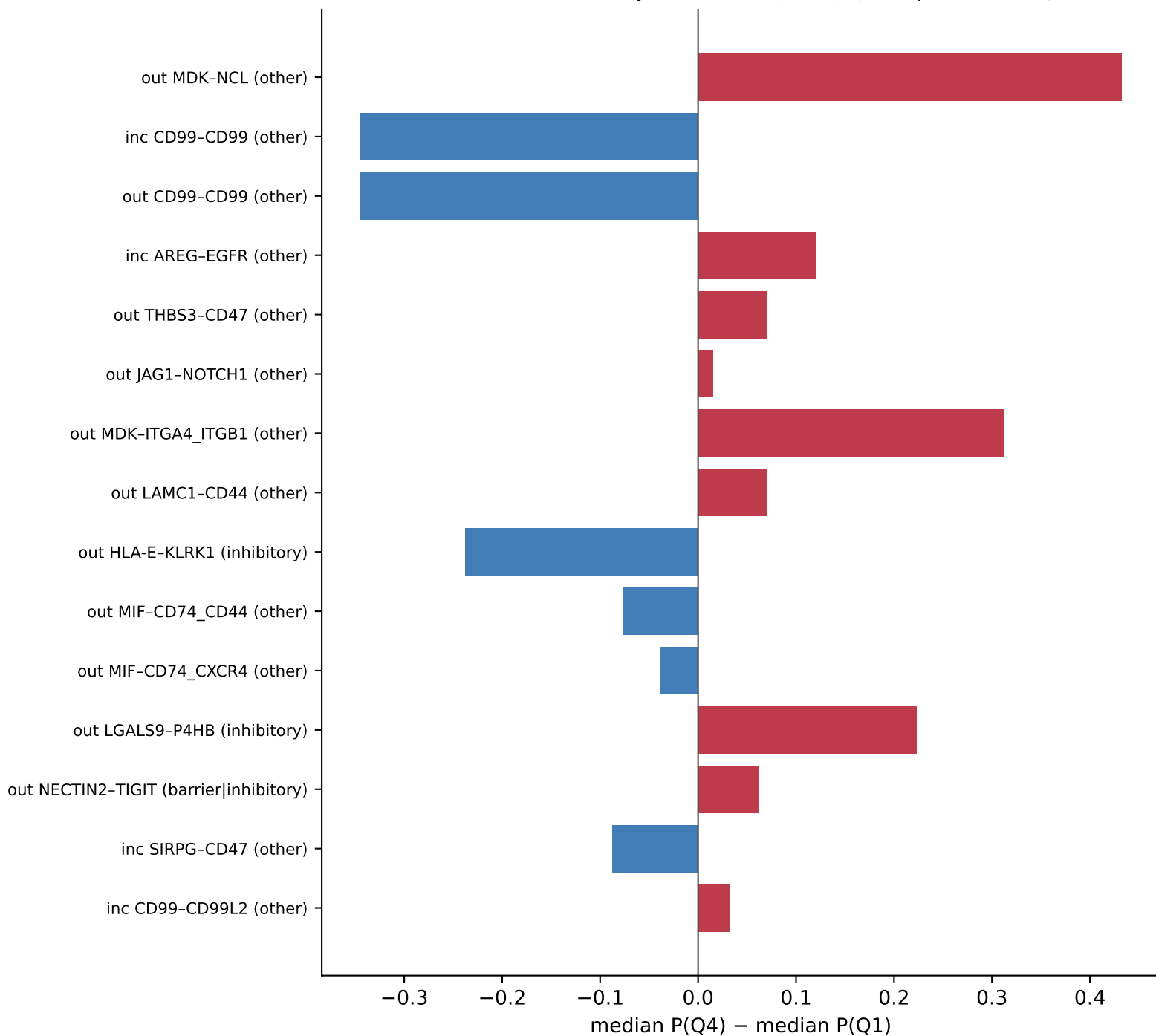
GSE205335 CellChat-style Mal↔T/NK Q4 vs Q1 (same-patient; n=6/6)
