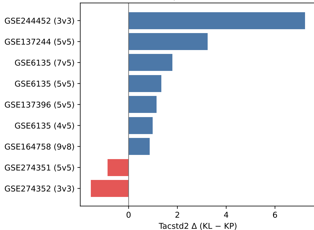
BULK: unadjusted Tacstd2 KL>KP
