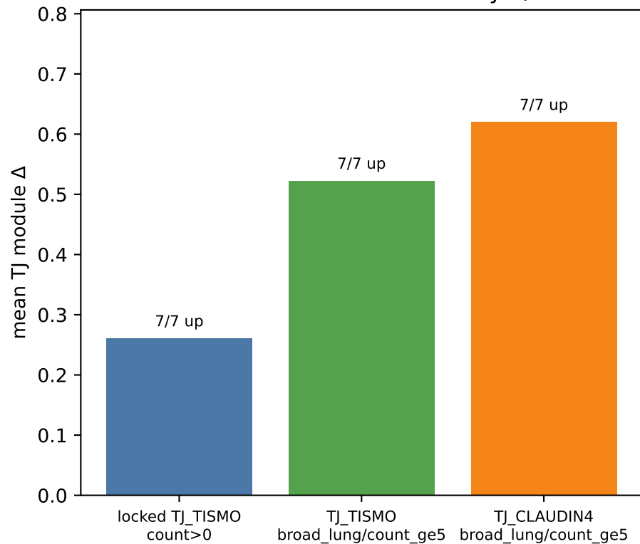
scRNA: concordance already 7/7
