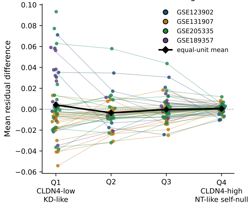
IFN minus detection-matched genes
