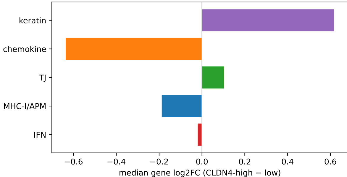
Family median logFC, combined Q4 vs Q1
