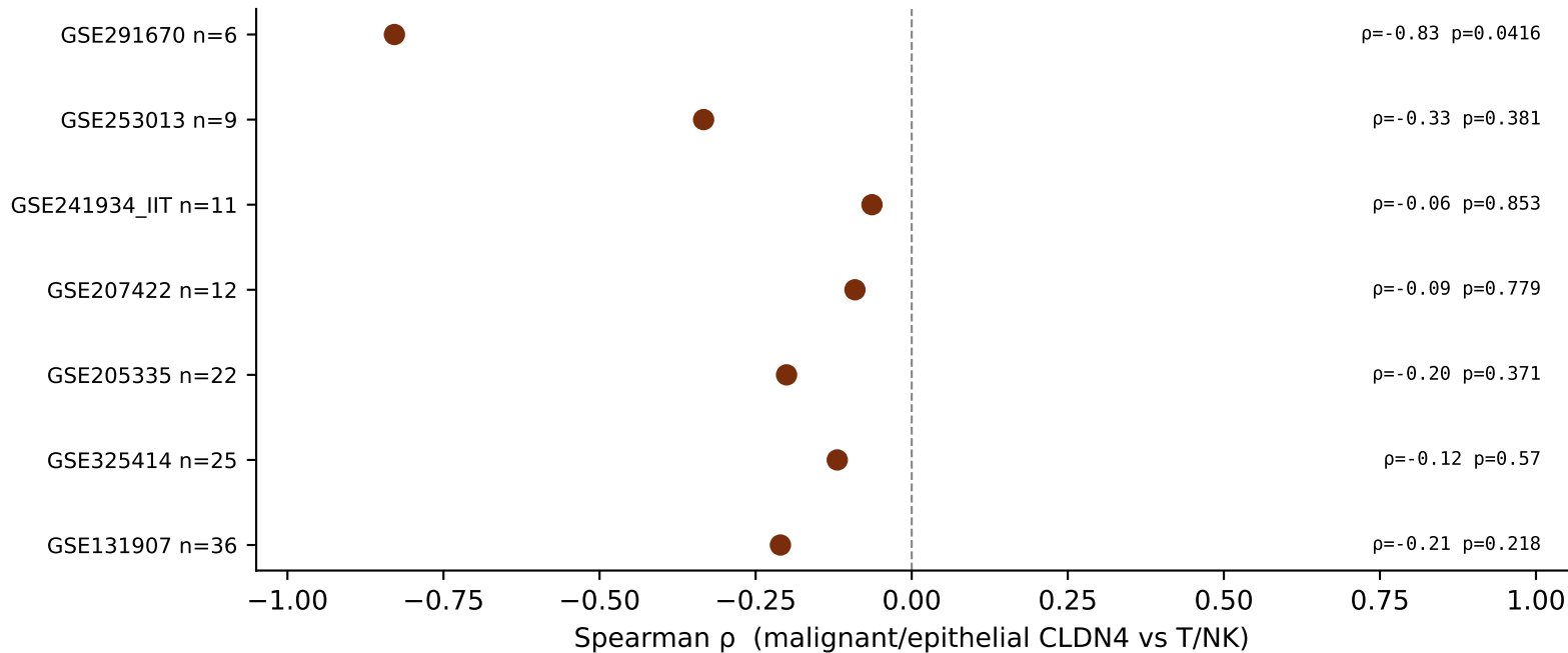
Primary-grid members with CLDN4 \rho < 0 vs T/NK
