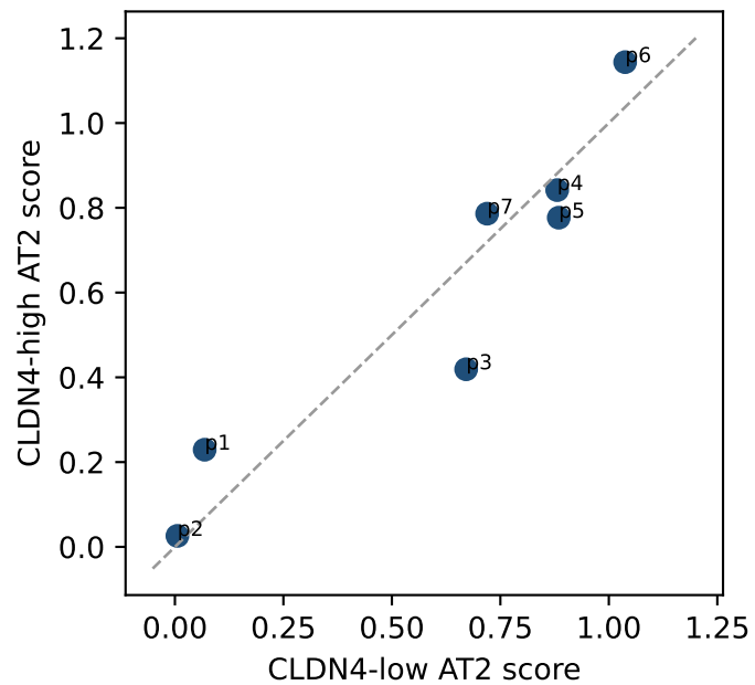
EXTRA: within-patient CLDN4-high vs low paired n=7 (n=7 thin)
