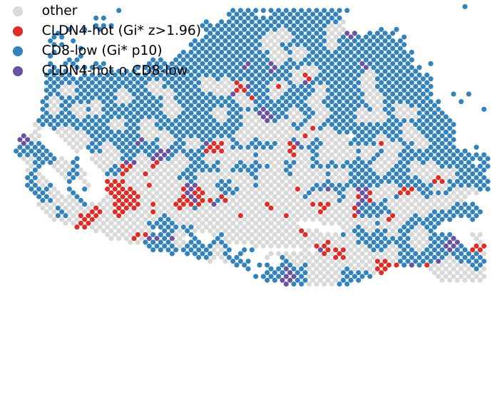
Gi* overlay I=+0.027 hotnCD8-low=69/3194
