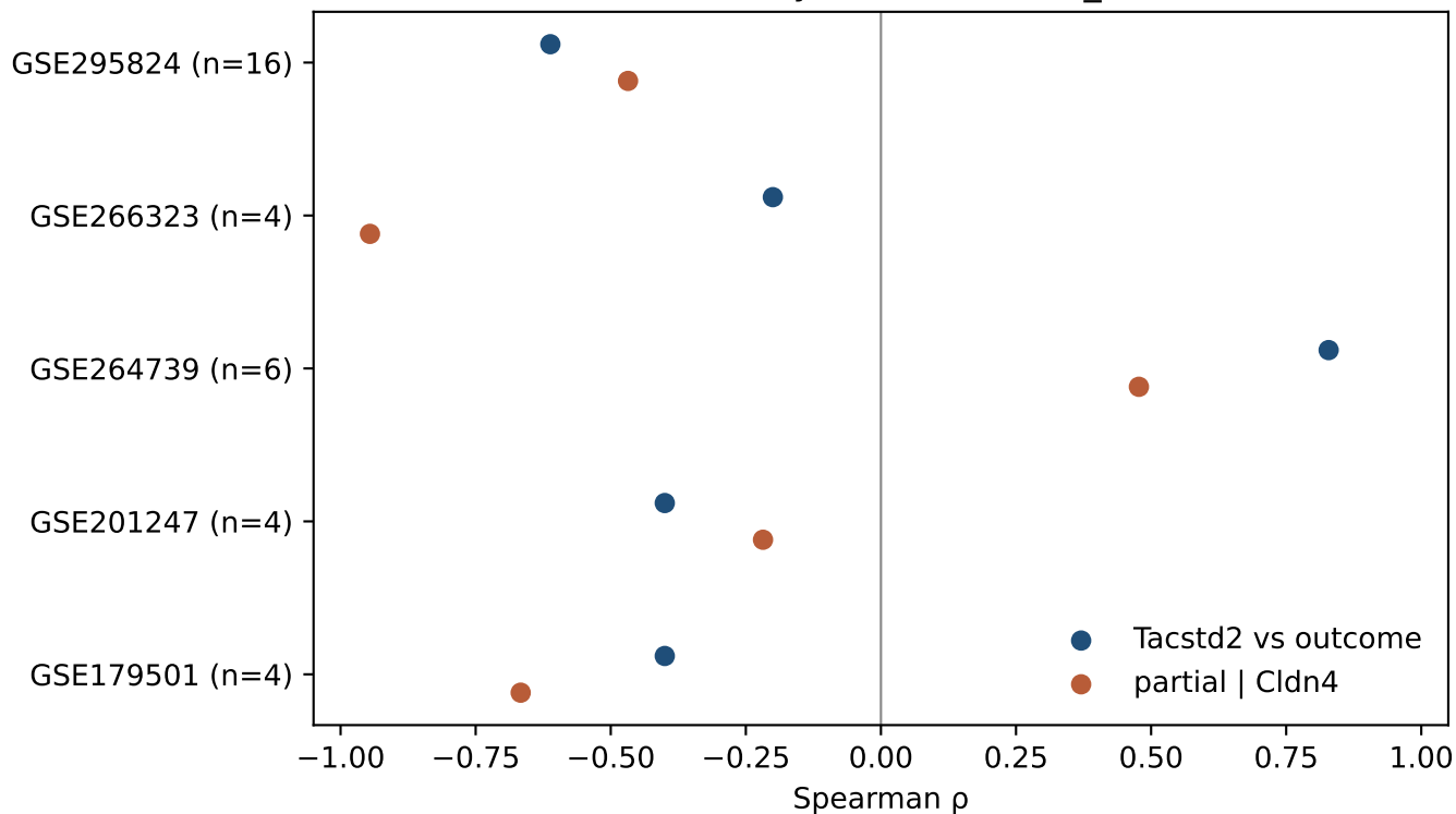
Within-study Tacstd2 % vs T_frac
