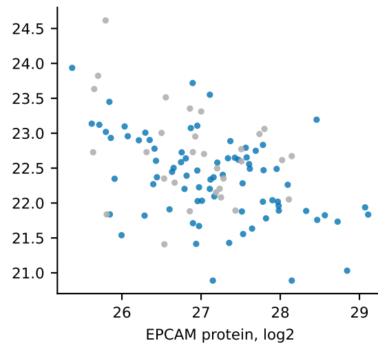
LSCC EPCAM vs CD8A \rho=-0.396 , n=108 , p=2.2e-05
