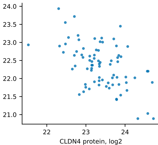
LSCC CLDN4 vs CD8A \rho=-0.444 , n=78 , p=4.6e-05
