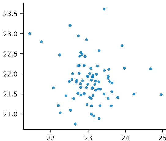
LSCC CLDN4 vs CD8A \rho=-0.444 , n=78 , p=4.6e-05
