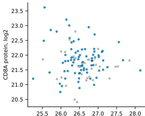
LSCC TACSTD2 vs CD8A \rho=-0.103 , n=108 , p=0.287
