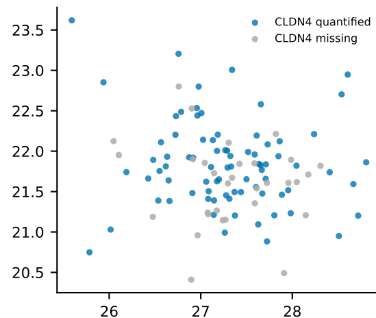
LSCC EPCAM vs CD8A \rho=-0.396 , n=108 , p=2.2e-05
