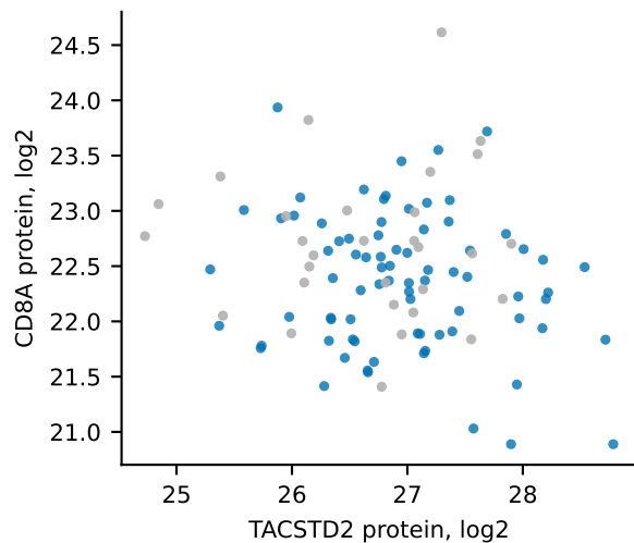
LSCC TACSTD2 vs CD8A \rho=-0.103 , n=108 , p=0.287
