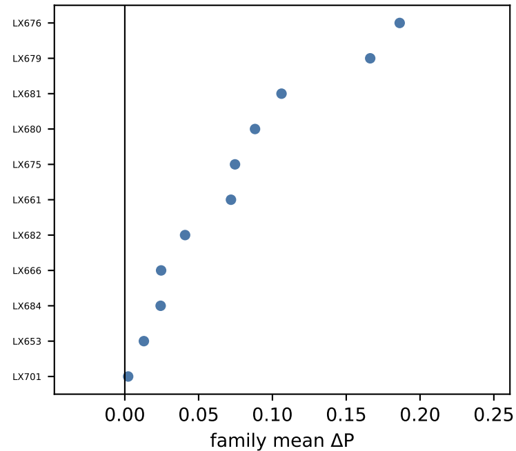
GSE123902
