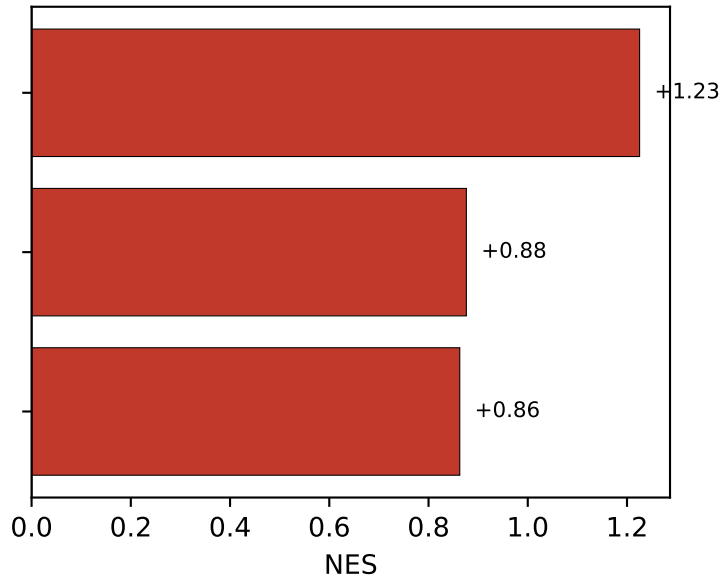
Sensitivity: Spearman vs CLDN4
