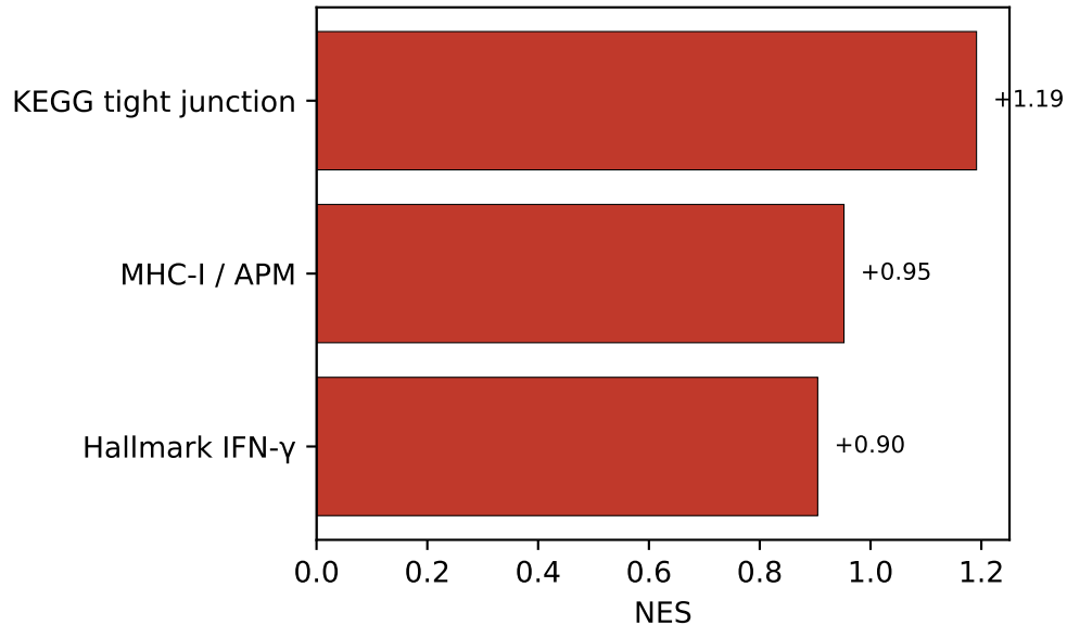
Primary: Welch t Q4–Q1
