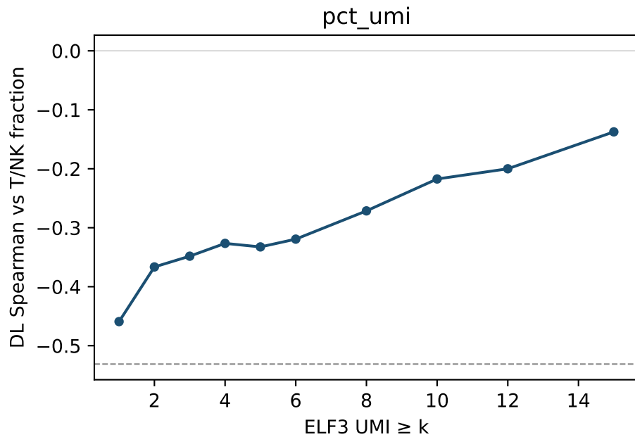
ELF3 score vs threshold (dashed = locked CLDN4 %pos)
