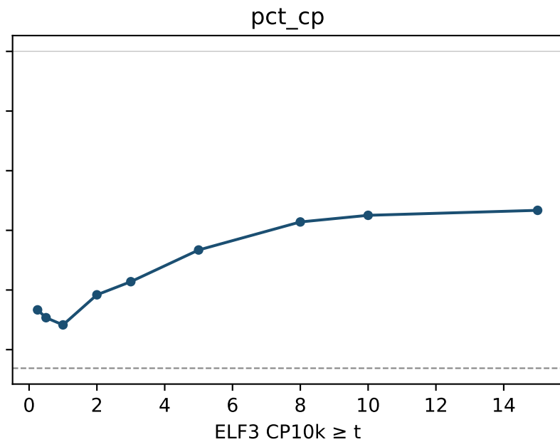
ELF3 score vs threshold (dashed = locked CLDN4 %pos)
