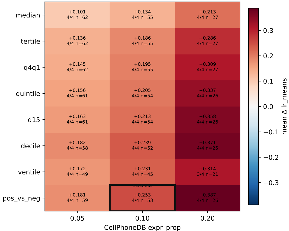
T/NK family mean \Delta (high – low)
