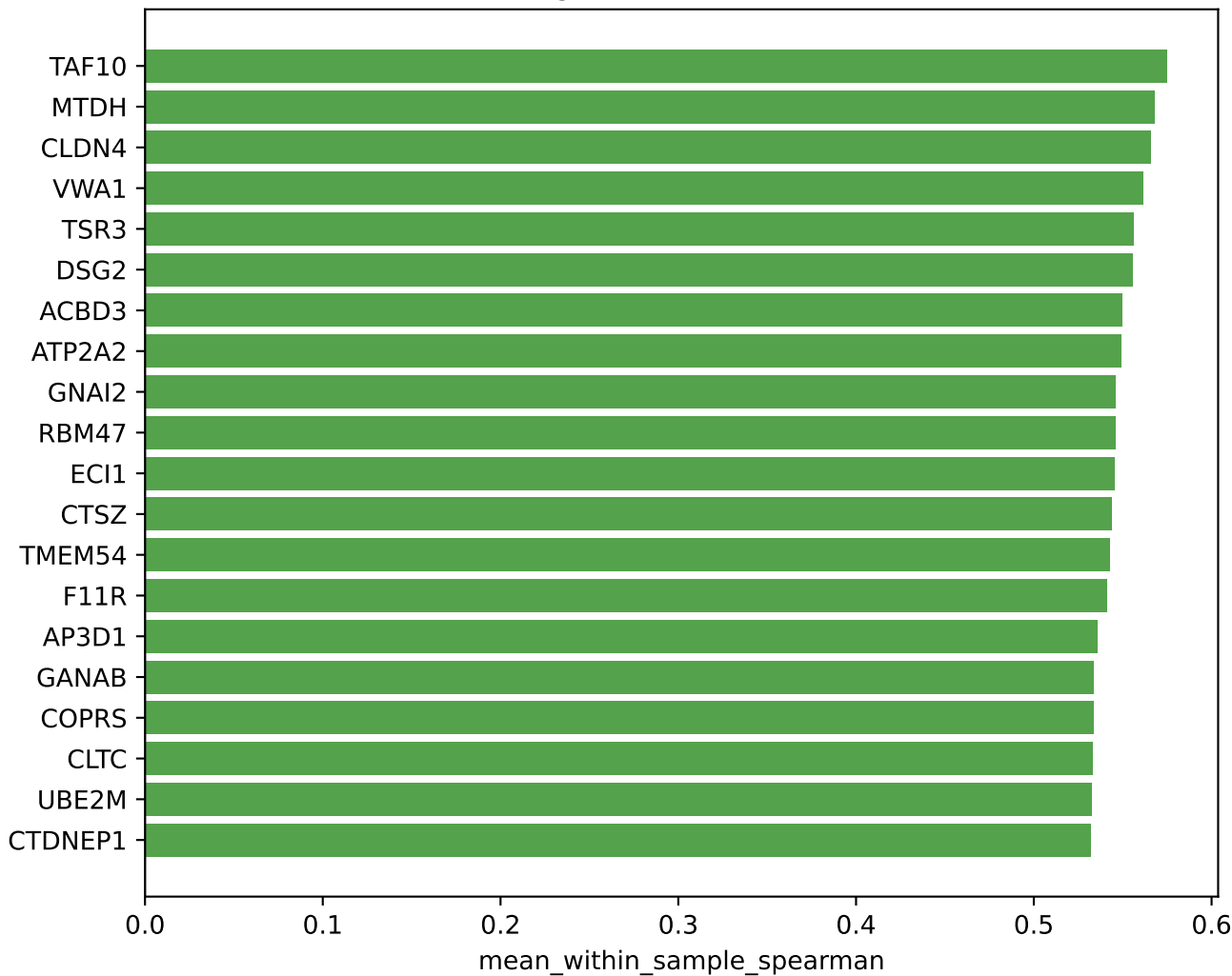
Genes tracking the Geneformer holdout axis
