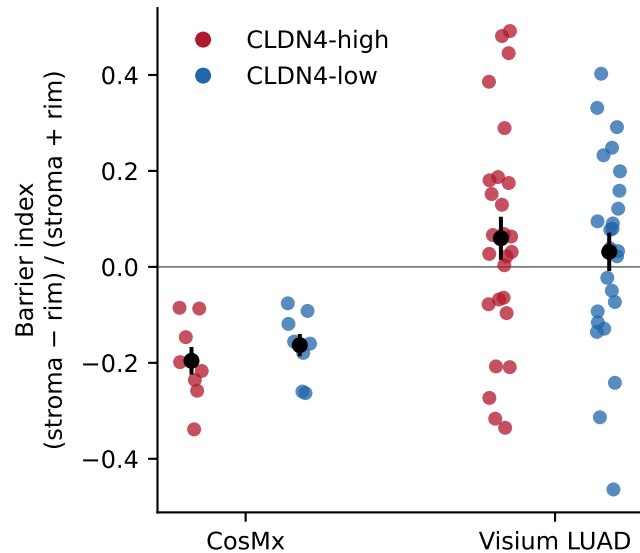
Barrier index at the CLDN4 rim
