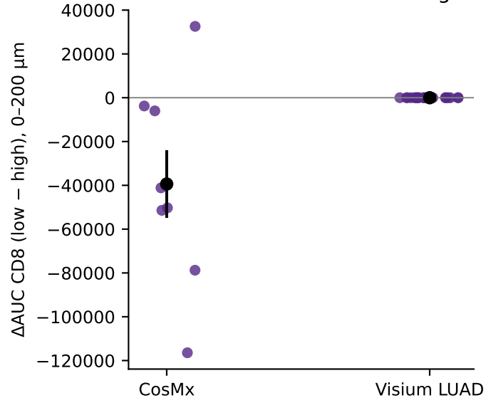
Infiltration AUC: low minus high
