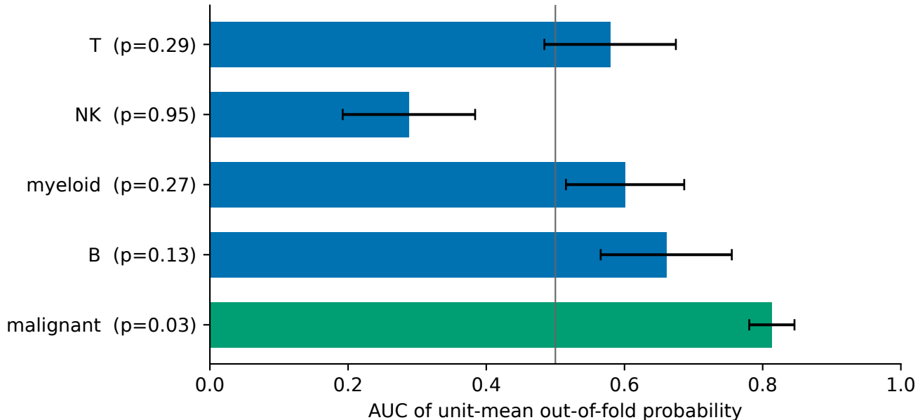
Augur-style priority, patient-blocked CV (n = 35 Q1/Q4 units)
