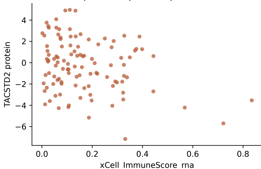
TACSTD2 protein vs xCell ImmuneScore Spearman \rho=-0.17 p=0.0713
