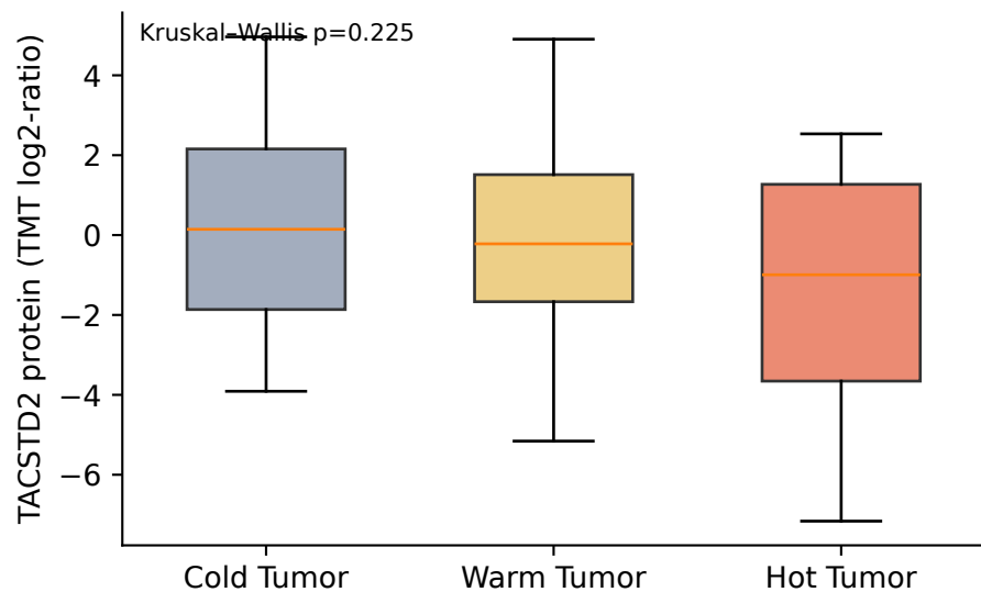
LSCC Immune.Cluster.rna (treatment-naive)
