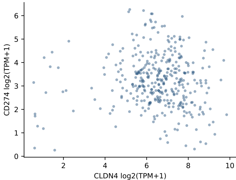
All tumors \rho=-0.112 p=0.0319 n=365
