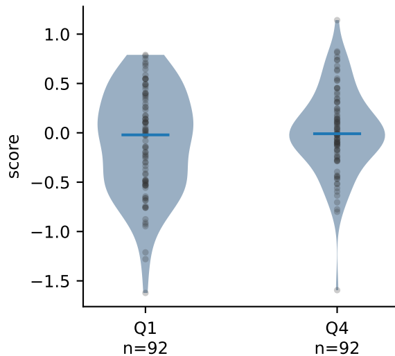
IFN- \gamma no MHC-I \delta = +0.11 p = 0.207
