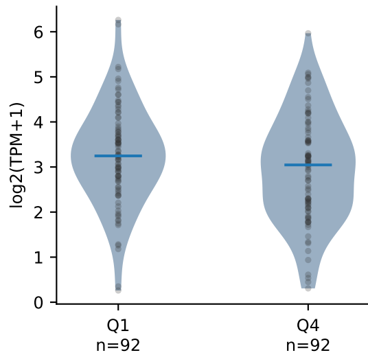
CD274 \delta = -0.16 p = 0.0671
