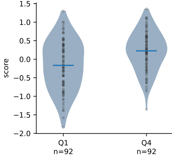
MHC-I/APM (known) \delta = +0.33 p = 0.000137
