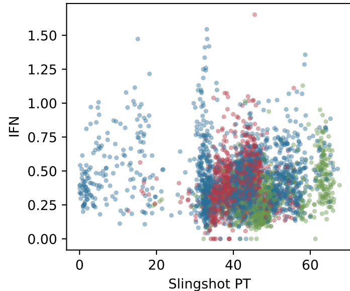
IFN along PT (cells; descriptive)
