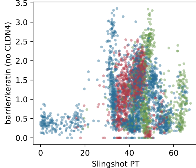
barrier/keratin (no CLDN4) along PT (cells; descriptive)
