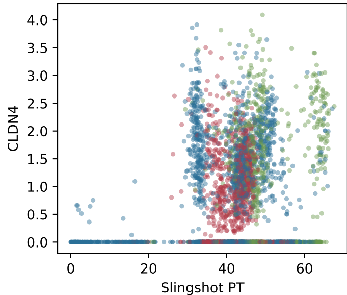
CLDN4 along PT (cells; descriptive)
