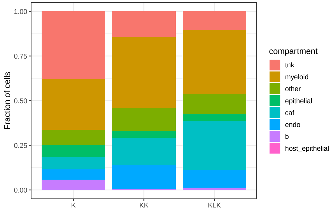
Marker compartments by genotype
