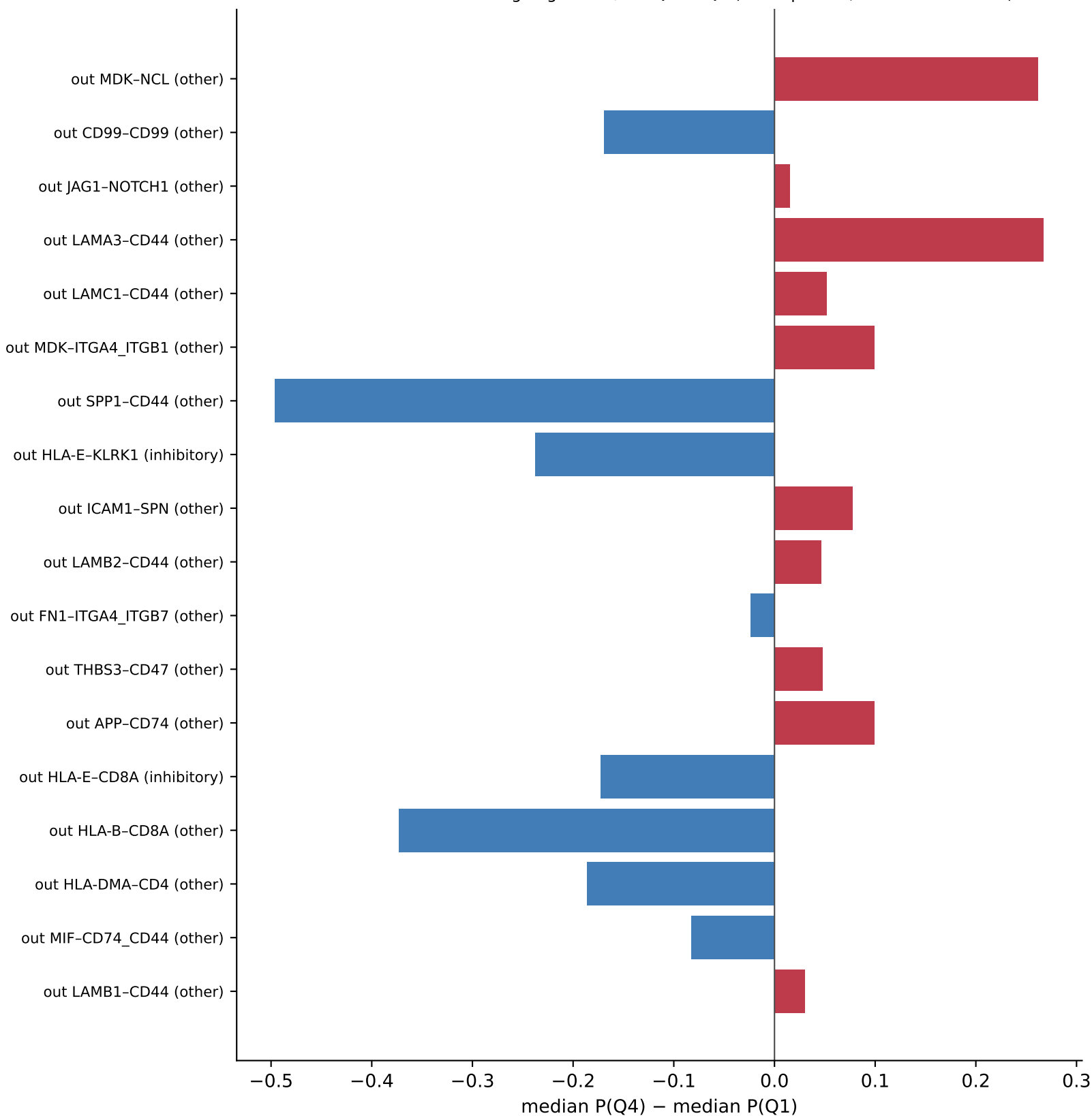
Pair 148071+205335 outgoing Mal→T/NK Q4 vs Q1 (same-patient; within-cohort tails)
