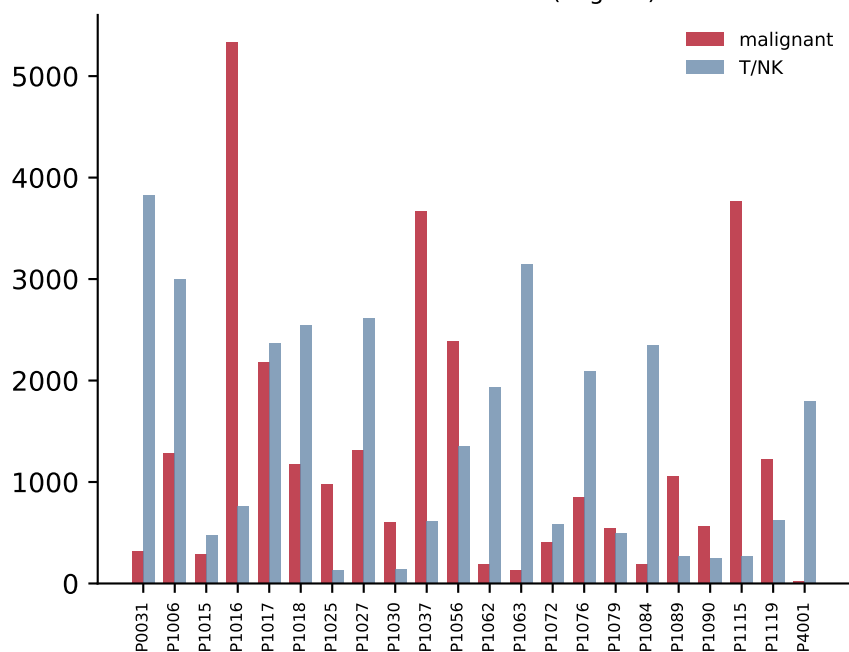
GSE205335 honest n (eligible)
