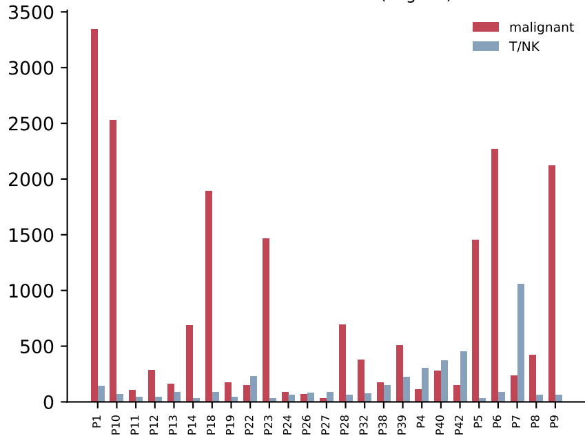
GSE148071 honest n (eligible)
