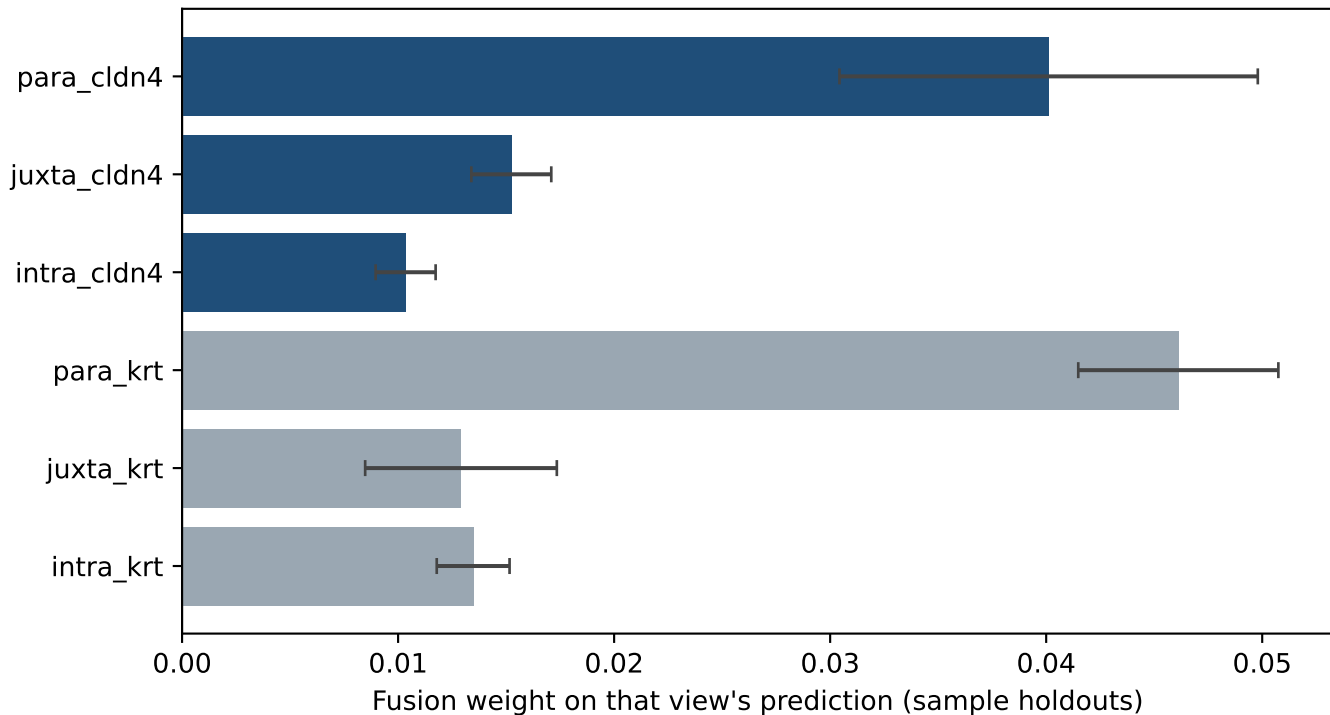
MISTy late-fusion weights, 50 \mu m CD8/NK density
