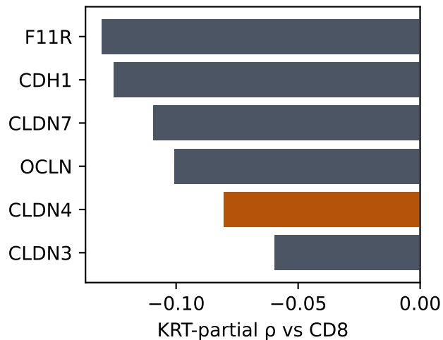
TCGA CLDN4 does not lead (0/60)
