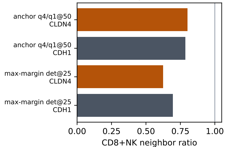
CosMx (CLDN3/7/OCLN/F11R OFF) CLDN4 wins only vs CDH1 at short
