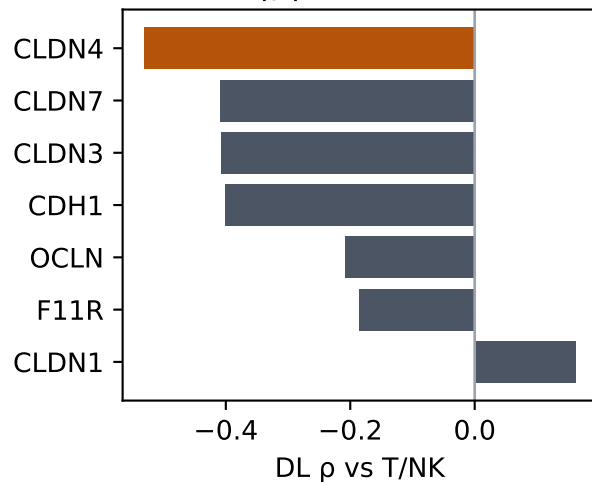
Concordant-4 max |\rho| (CLDN4 leads)
