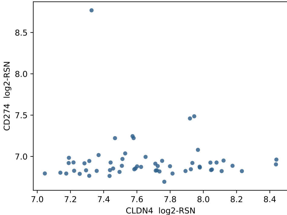
GSE32863 LUAD tumor CLDN4 vs CD274 n=58 \rho=+0.130 p=0.332
