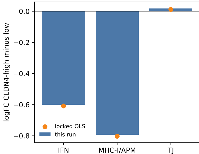
Observed malignant contrast
