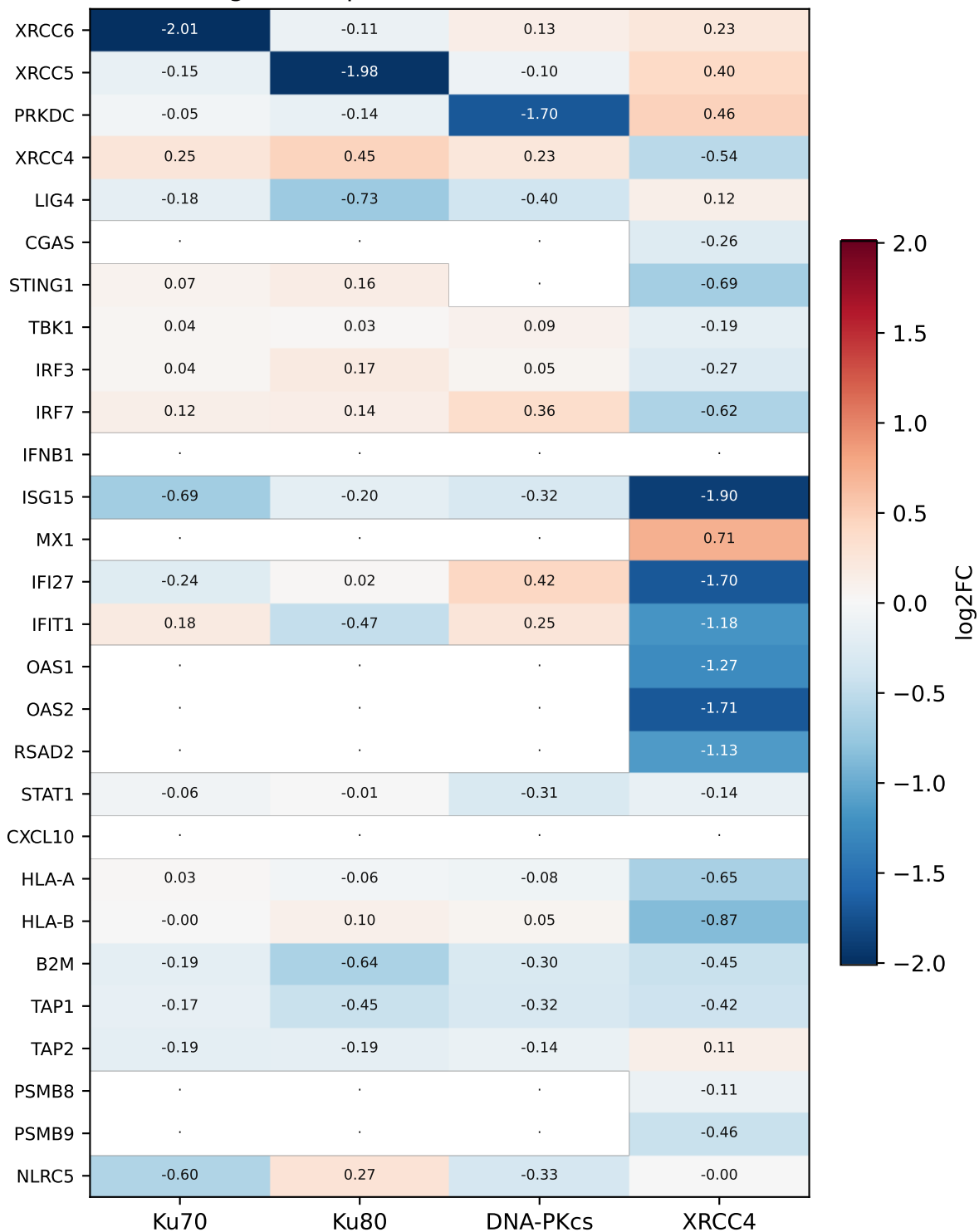
log2FC, depleted vs matched control
