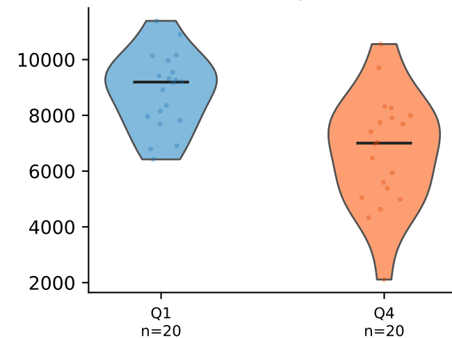
CPTAC-LSCC-protein \delta=-2.19e+03 p=0.001
