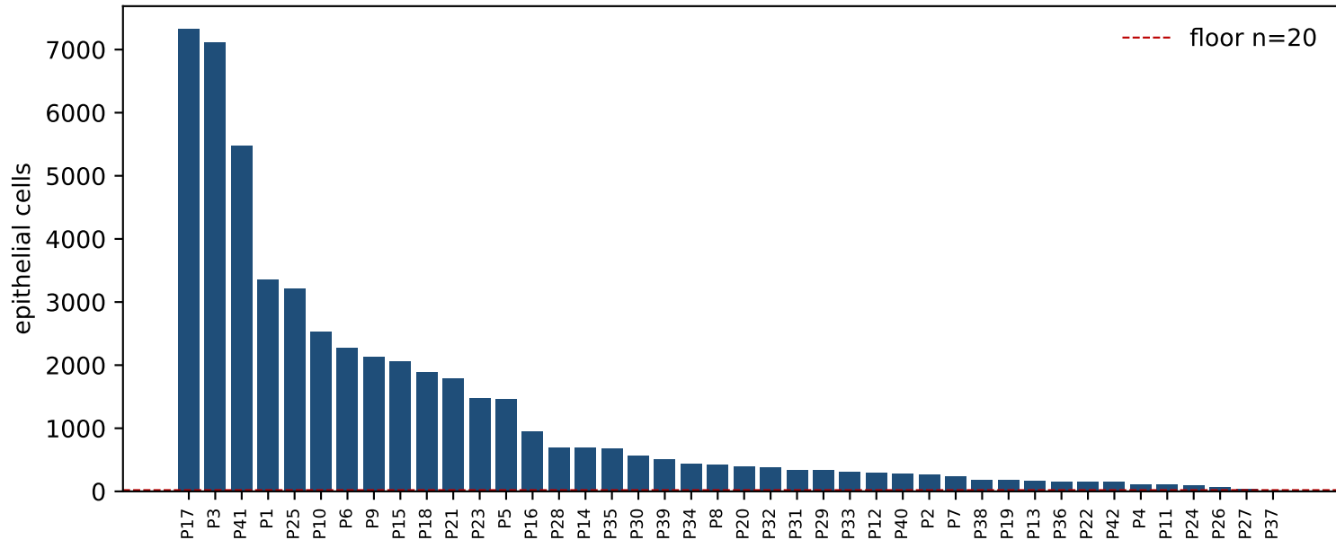
GSE148071 honest n — epithelial occupancy (blue = eligible)
